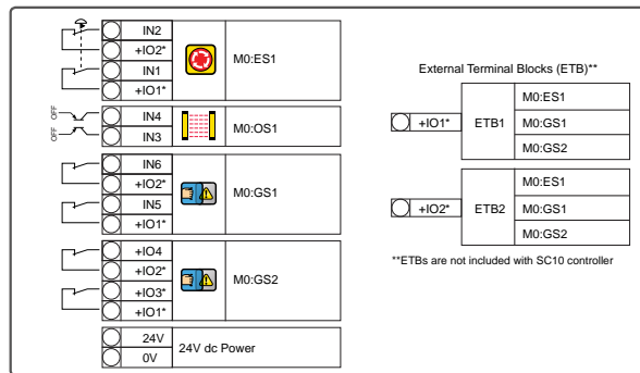
Wire Diagram View for 14 Inputs with ATO
