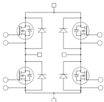
Full Bridge
