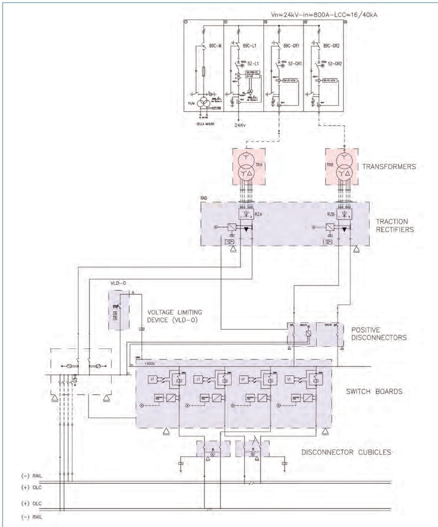
Typical schematic of a traction electrical substation
