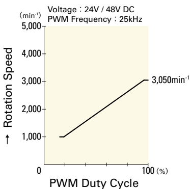
9B1TP24P0H001 9B1TP48P0H001
