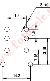
PCB Mounting
