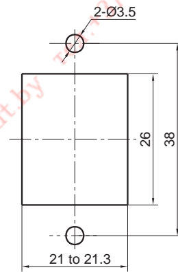
PCB layout
