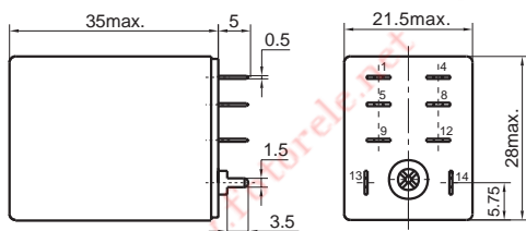
Outline Dimensions
