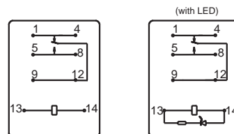
Wiring Diagram
